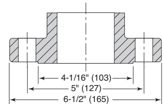
2" (51) ANSI, 250 lb. (113 kg) 8-Bolt Flange
