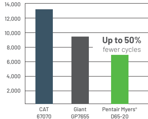
CRANK REVOLUTIONS TO PUMP 1000 GALLONS
